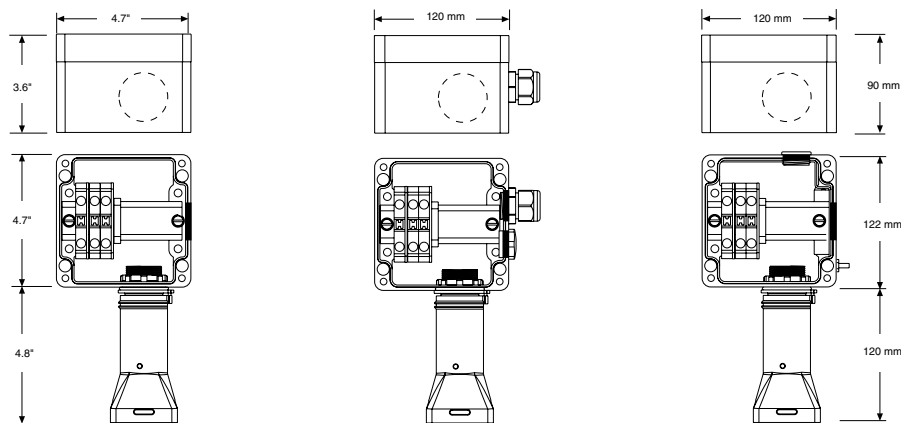
JBS-100-A JBS-100-L-A
